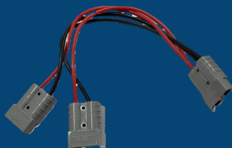
50 Amp Connector Plug Split 300mm EP011
