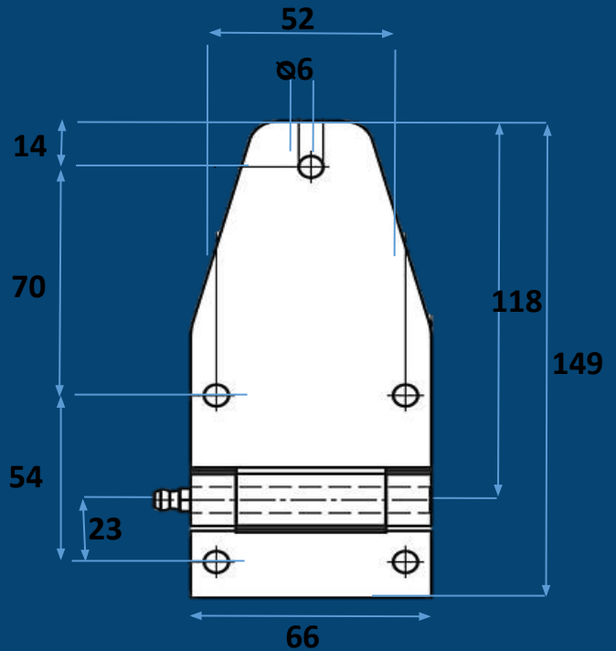
Heavy Duty Flap Hinge 5-hole Hinge Size: 66 x 149mm
