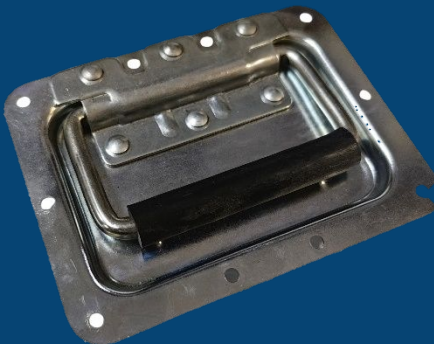
Recessed Spring-loaded Carry Handle Size: 147 x 110mm Stock Code: HC04
