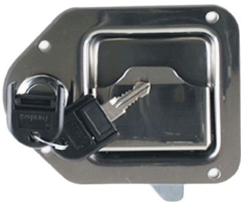
Small Paddle Handle - 83x111 Stainless Steel L13-002
